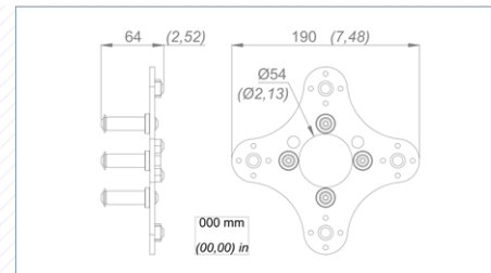
SUA034 (190 MM DRIVE PLATE)
