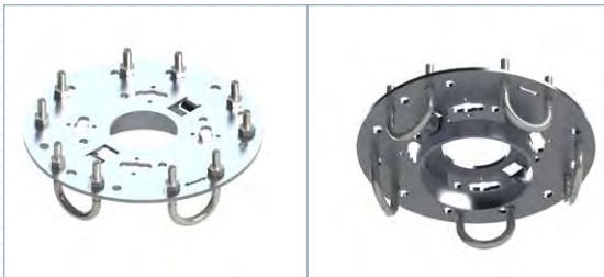
FUA001 FOR FLAT OR SLIGHTLY TAPERED HANDWHEELS (<30°)
